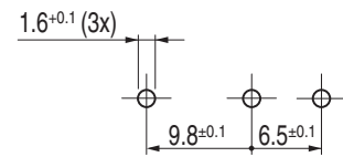
PCB Terminal Mounting Holes
