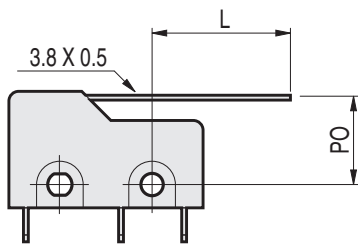
Hinge Lever (Type G)
