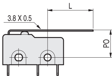
Hinge Lever (Type E)
