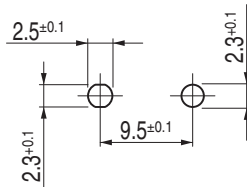
Mounting Holes
