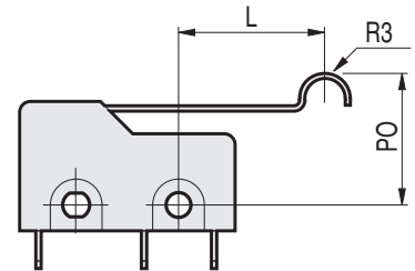
Roller Simulated Hinge Lever (Type D)
