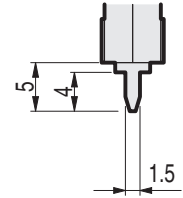
PCB Terminal
