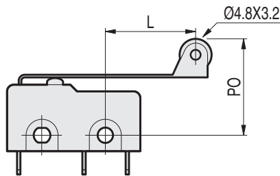
Roller Hinge Lever (Type R)
