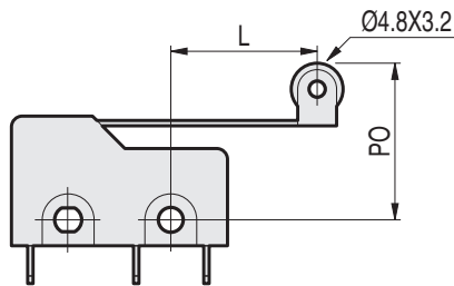
Roller Hinge Lever (Type J)
