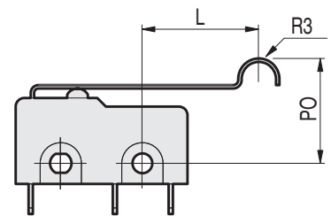
Roller Simulated Hinge Lever (Type U)
